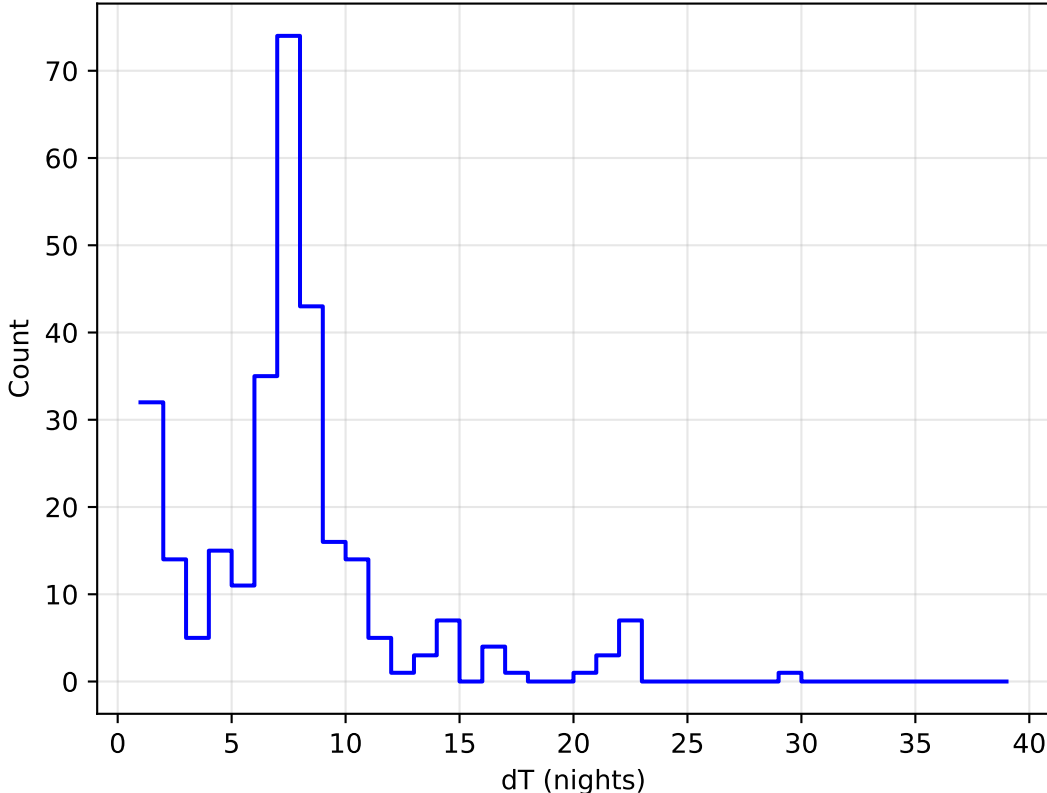
roll_uniform_early_half_mjdp0_v3.4_10yrs all bands: DD:EDFS Delta Nights Histogram
