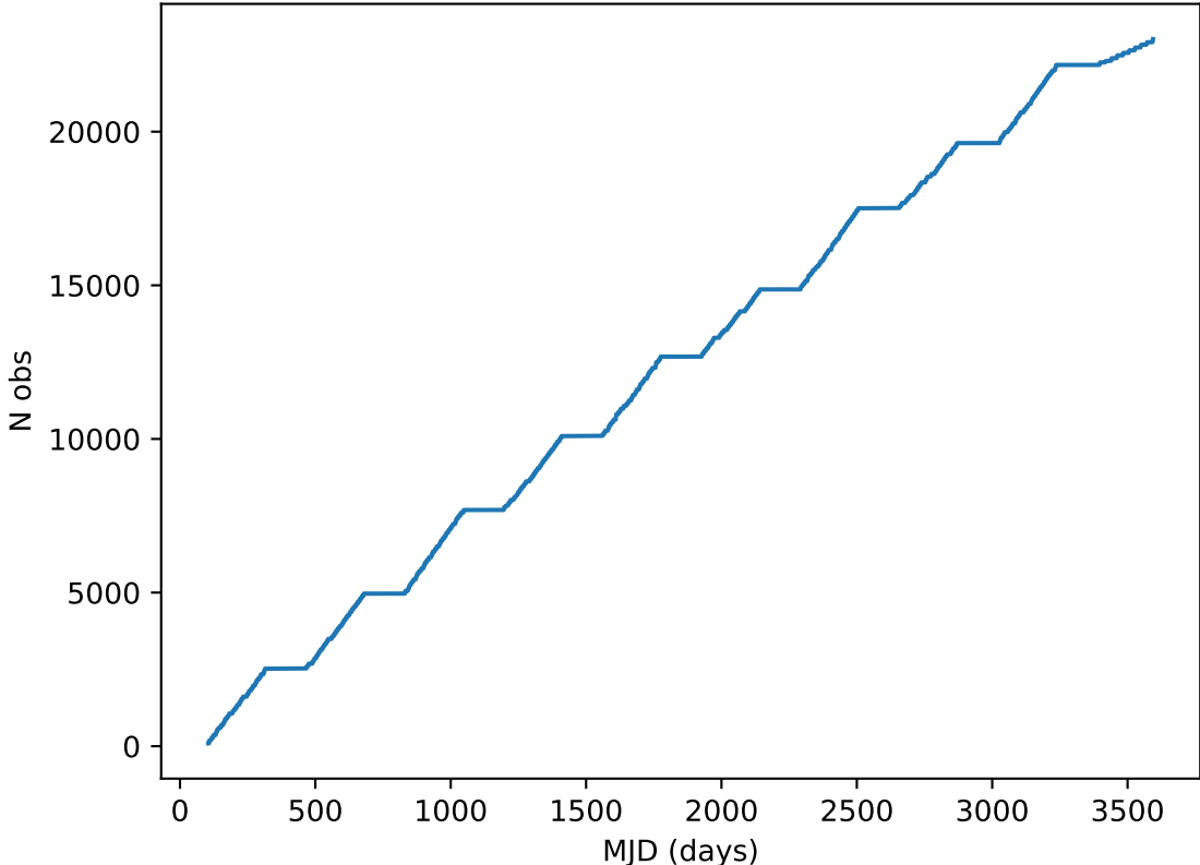
roll_uniform_early_half_mjdp0_v3.4_10yrs all bands: DD:EDFS Cumulative NVisits
