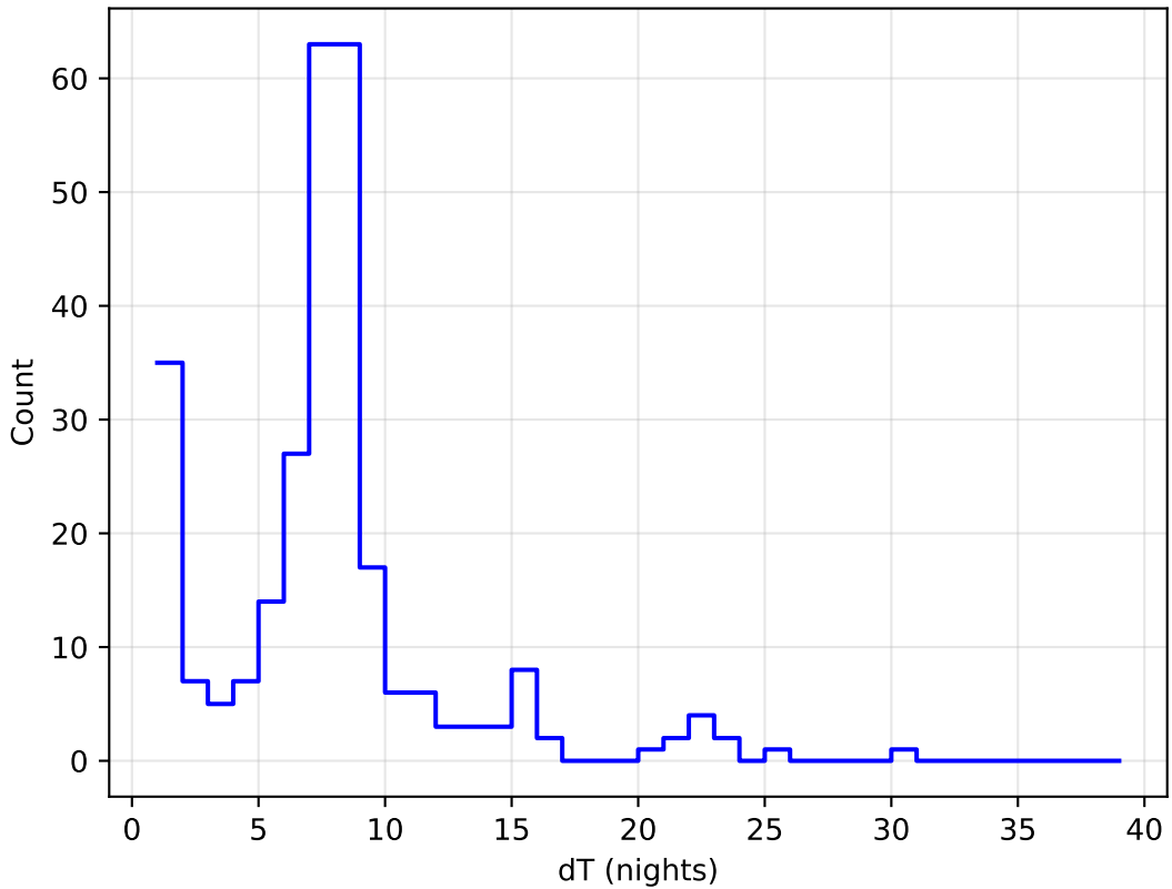
roll_uniform_early_half_mjdp0_v3.4_10yrs all bands: DD:ECDFS Delta Nights Histogram
