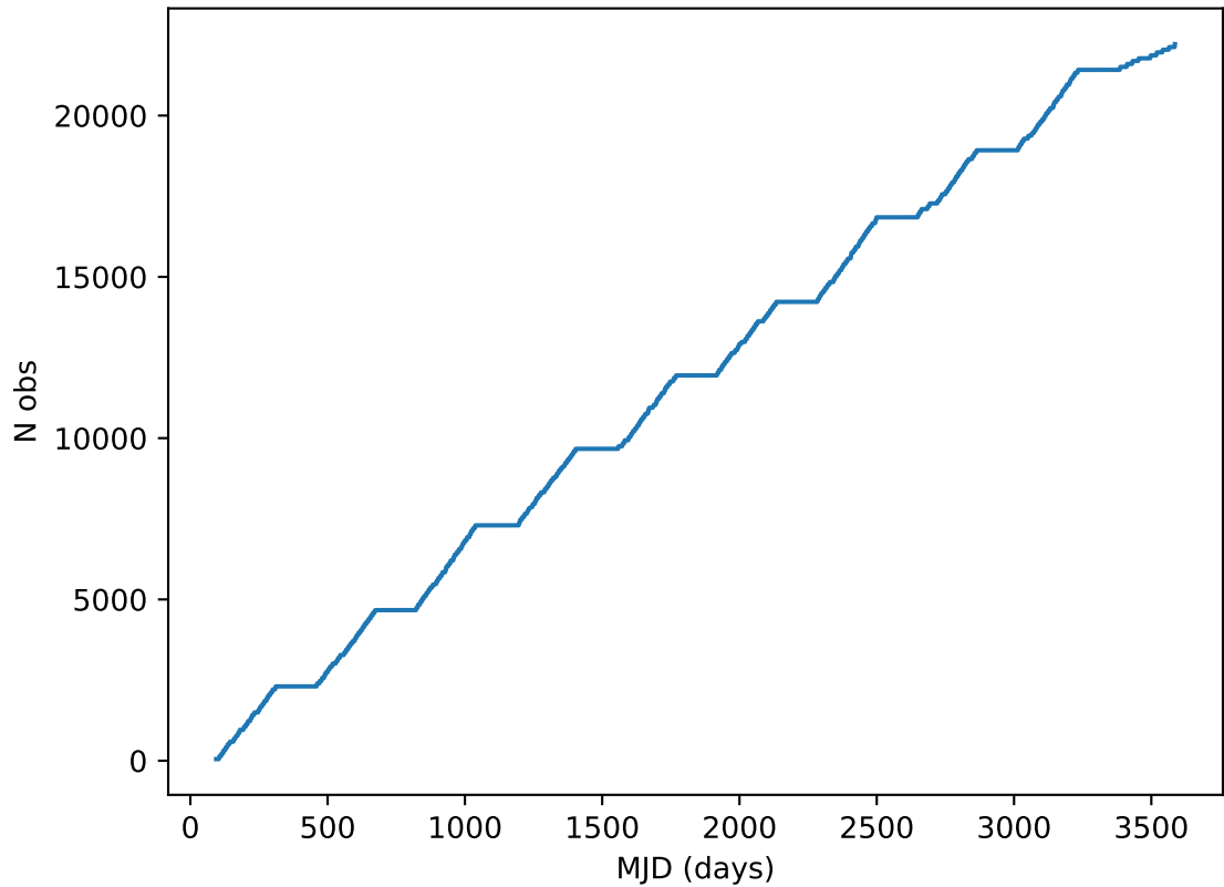
roll_uniform_early_half_mjdp0_v3.4_10yrs all bands: DD:ECDFS Cumulative NVisits
