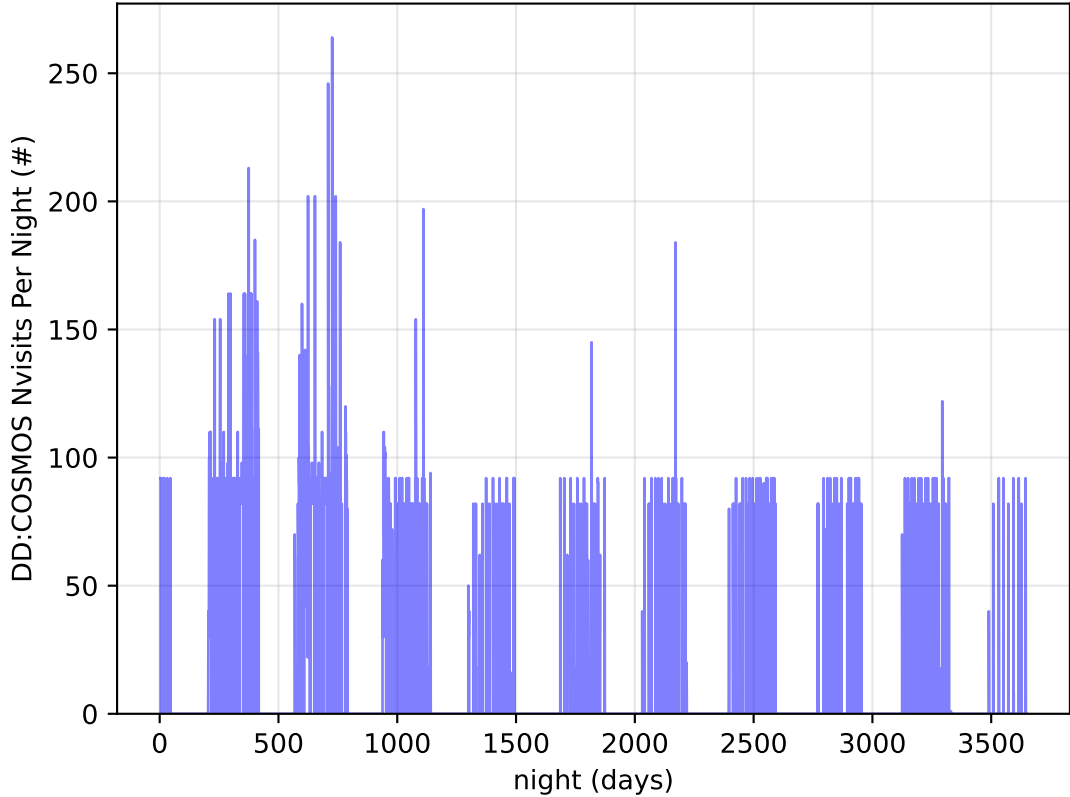
roll_uniform_early_half_mjdp0_v3.4_10yrs all bands: DD: COSMOS Nvisits Per Night
