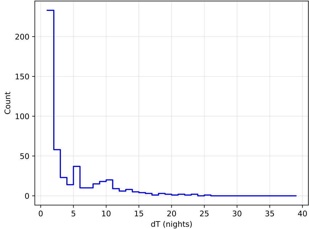
roll_uniform_early_half_mjdp0_v3.4_10yrs all bands: DD: COSMOS Delta Nights Histogram
