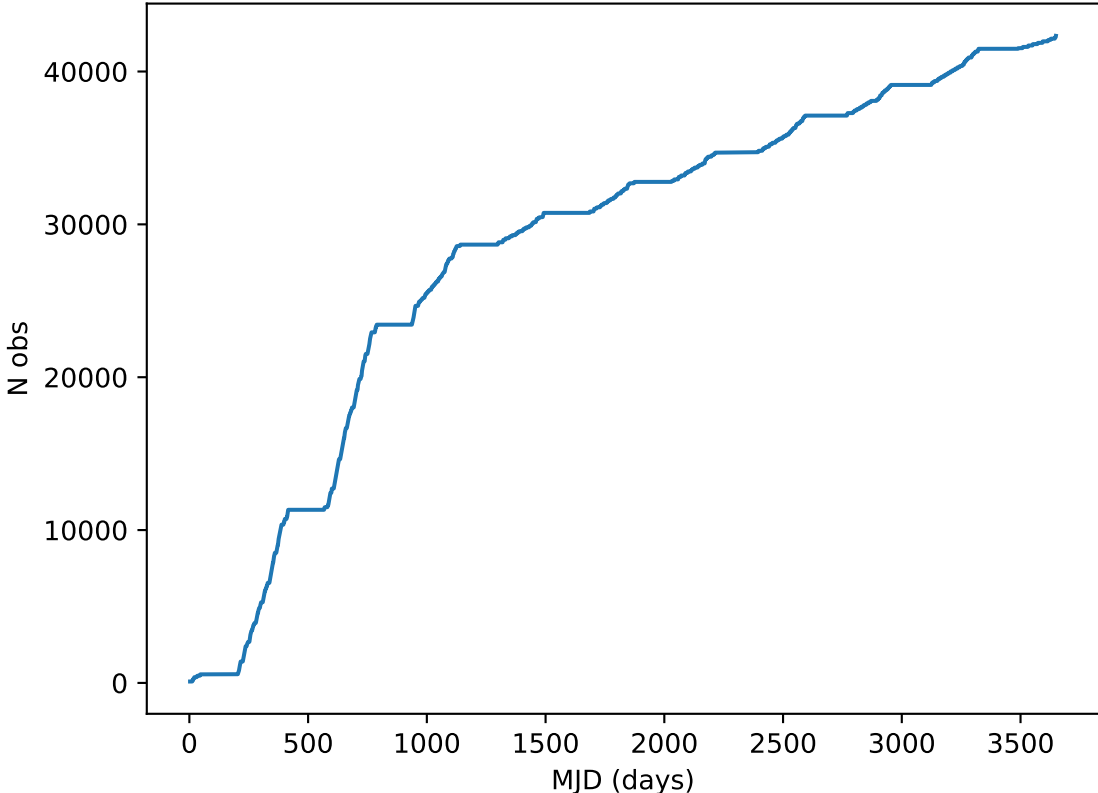
roll_uniform_early_half_mjdp0_v3.4_10yrs all bands: DD:COSMOS Cumulative NVisits
