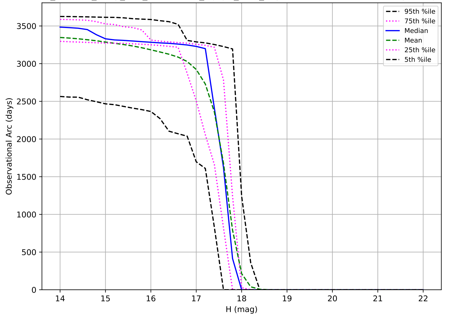
roll_uniform_early_half_accordion1_mjdp0_v3.4_10yrs: Observational Arc Length Trojan
