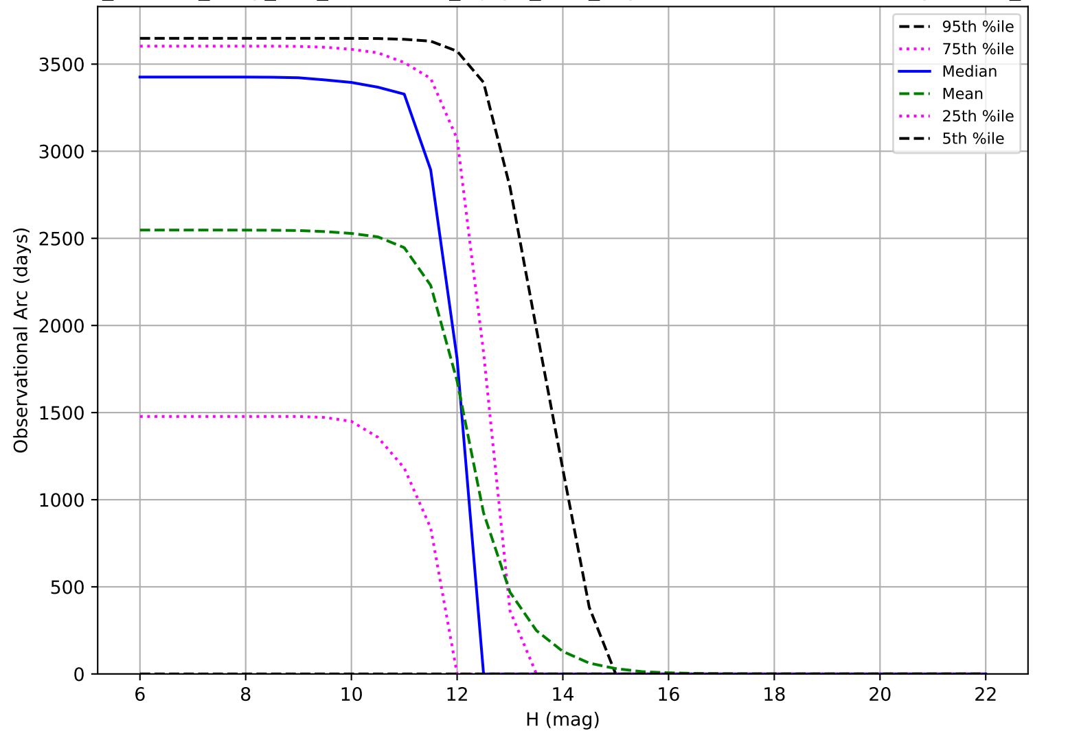
roll_uniform_early_half_accordion1_mjdp0_v3.4_10yrs: Observational Arc Length OCC_r20
