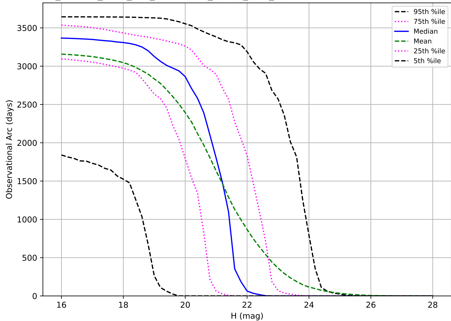
roll_uniform_early_half_accordion1_mjdp0_v3.4_10yrs: Observational Arc Length NEO
