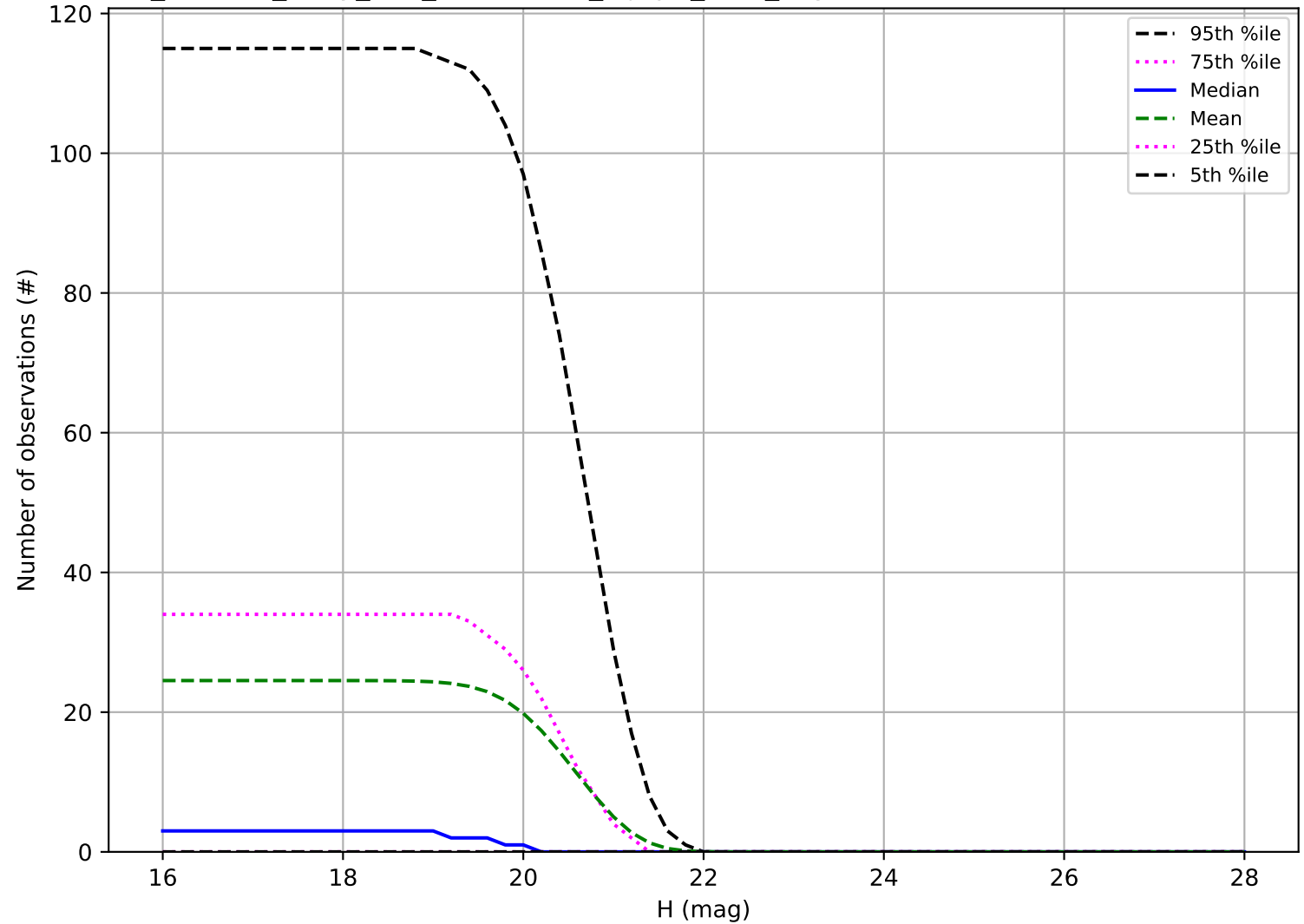
roll_uniform_early_half_accordion1_mjdp0_v3.4_10yrs: Number of observations Vatra
