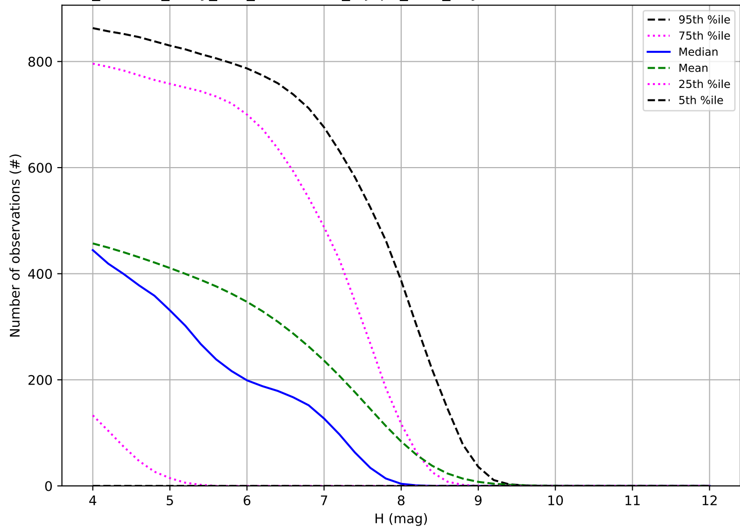
roll_uniform_early_half_accordion1_mjdp0_v3.4_10yrs: Number of observations TNO
