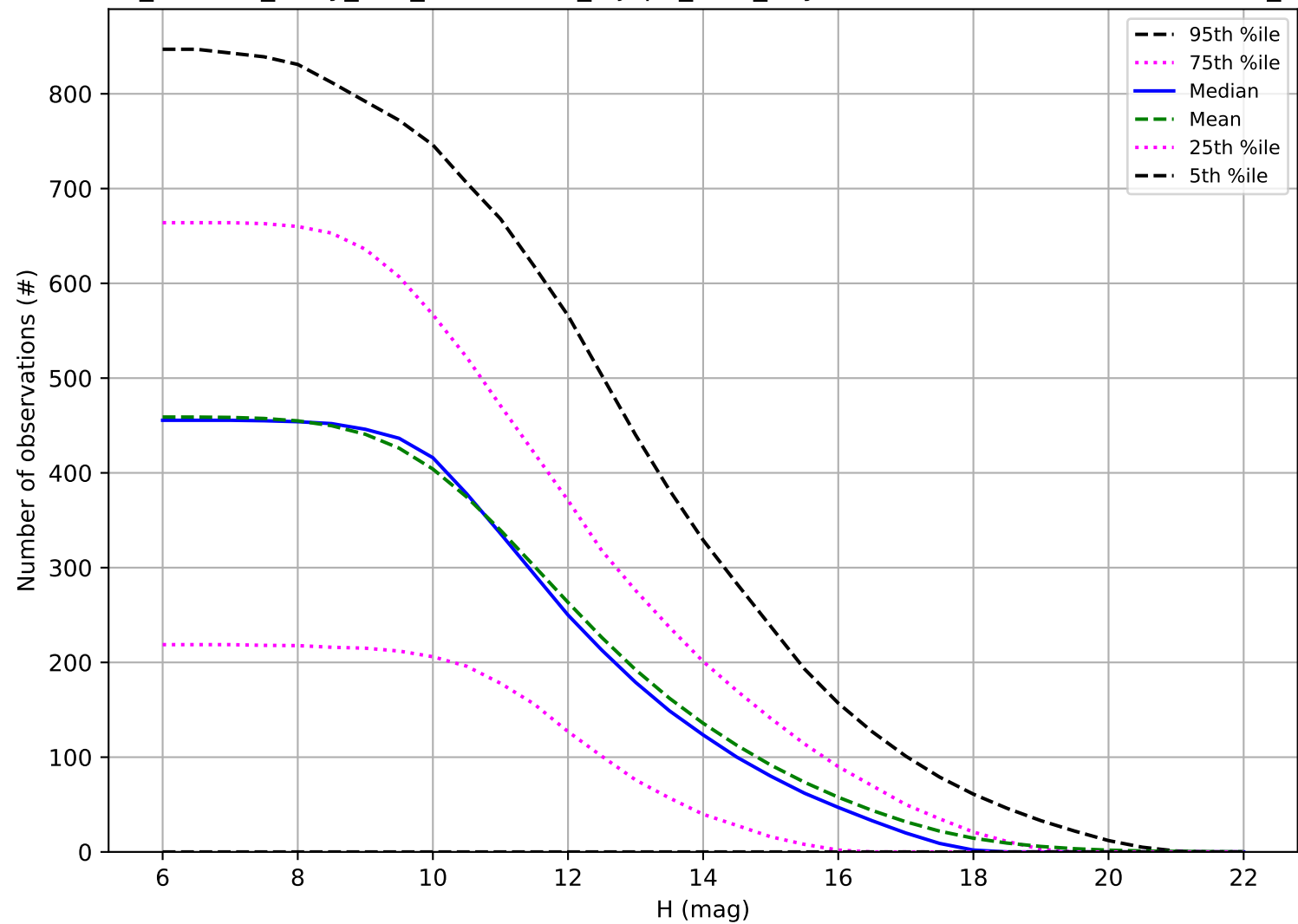
roll_uniform_early_half_accordion1_mjdp0_v3.4_10yrs: Number of observations OCC_r5
