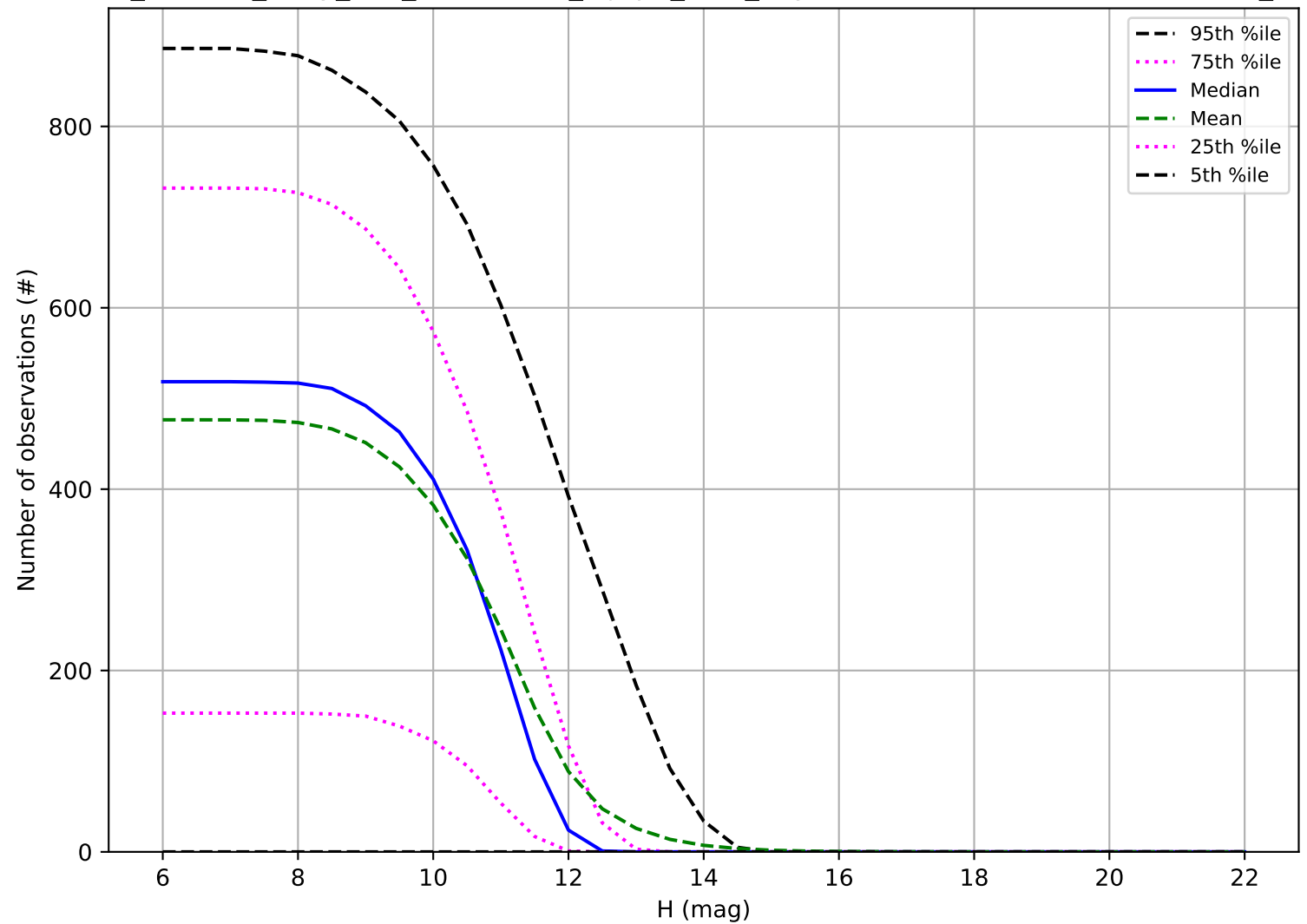
roll_uniform_early_half_accordion1_mjdp0_v3.4_10yrs: Number of observations OCC_r20
