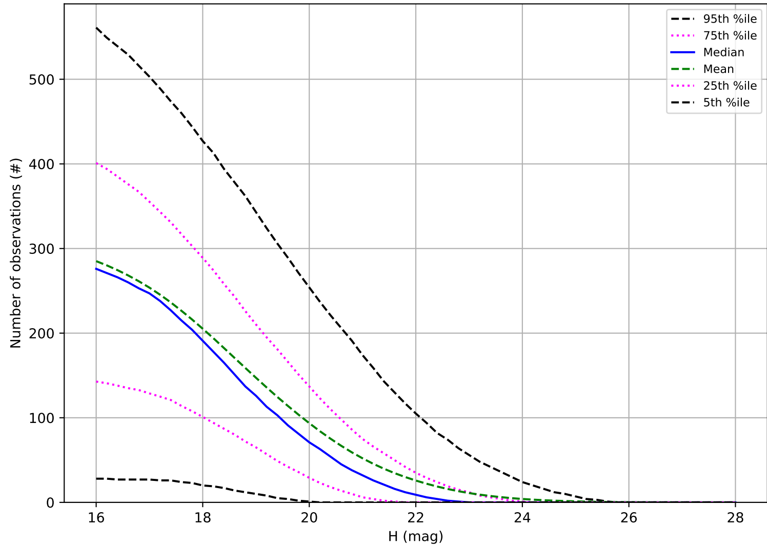
roll_uniform_early_half_accordion1_mjdp0_v3.4_10yrs: Number of observations NEO
