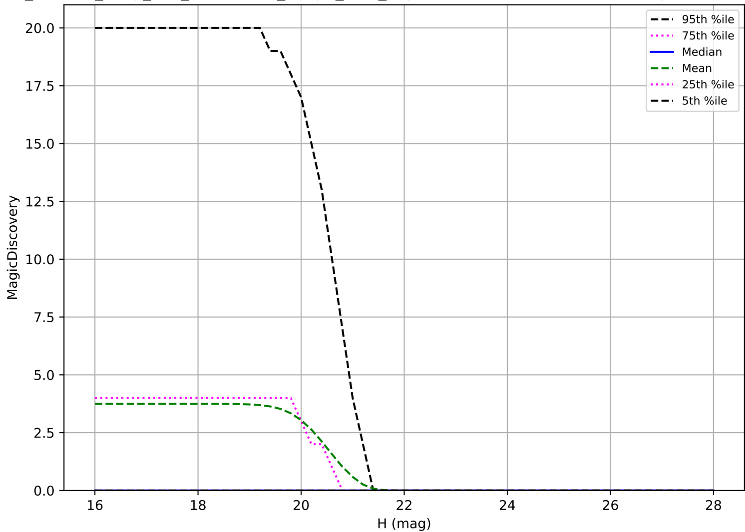
roll_uniform_early_half_accordion1_mjdp0_v3.4_10yrs: Vatira 6 detections in 60 nights detection loss
