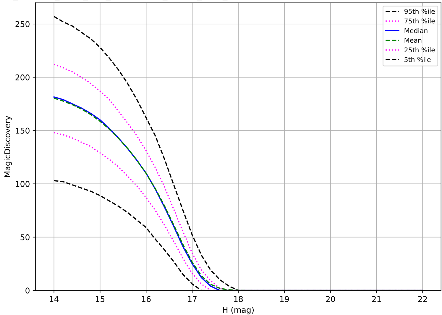
roll_uniform_early_half_accordion1_mjdp0_v3.4_10yrs: Trojan 6 detections in 60 nights detection loss
