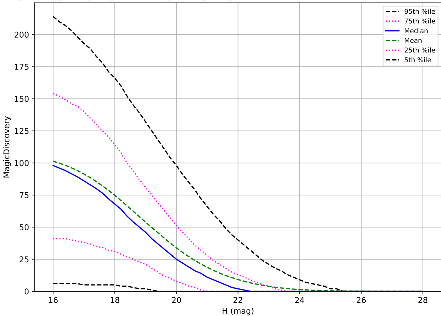
roll_uniform_early_half_accordion1_mjdp0_v3.4_10yrs: PHA 6 detections in 60 nights detection loss
