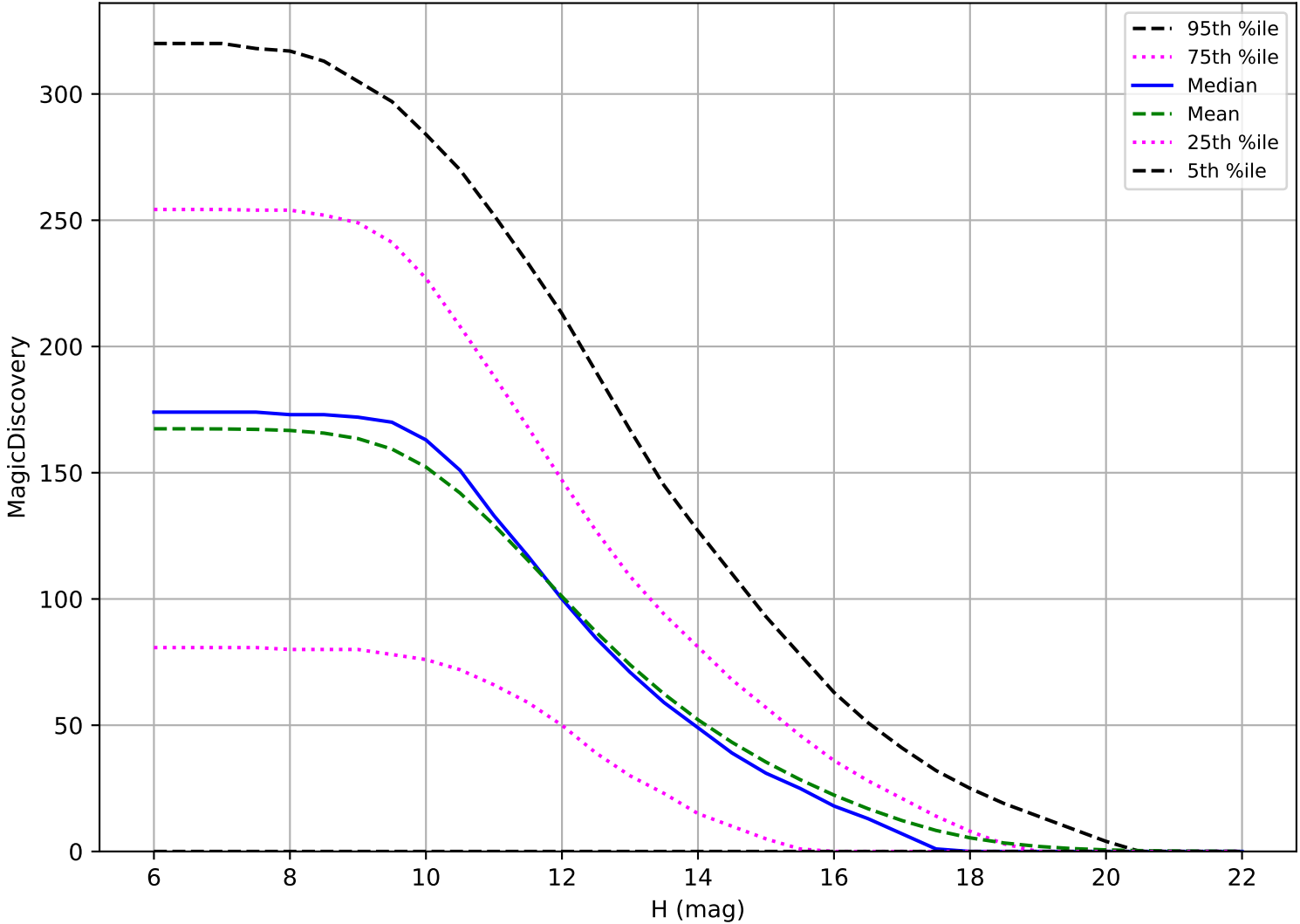
roll_uniform_early_half_accordion1_mjdp0_v3.4_10yrs: OCC_r5 6 detections in 60 nights detection loss
