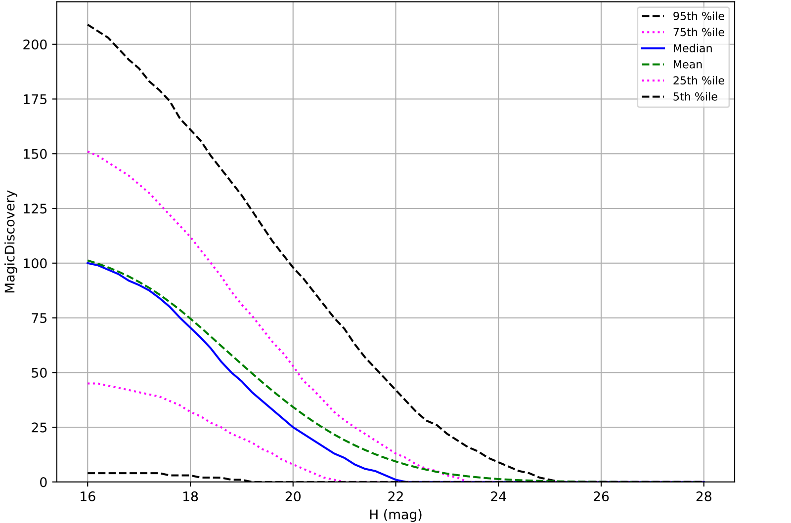
roll_uniform_early_half_accordion1_mjdp0_v3.4_10yrs: NEO 6 detections in 60 nights detection loss
