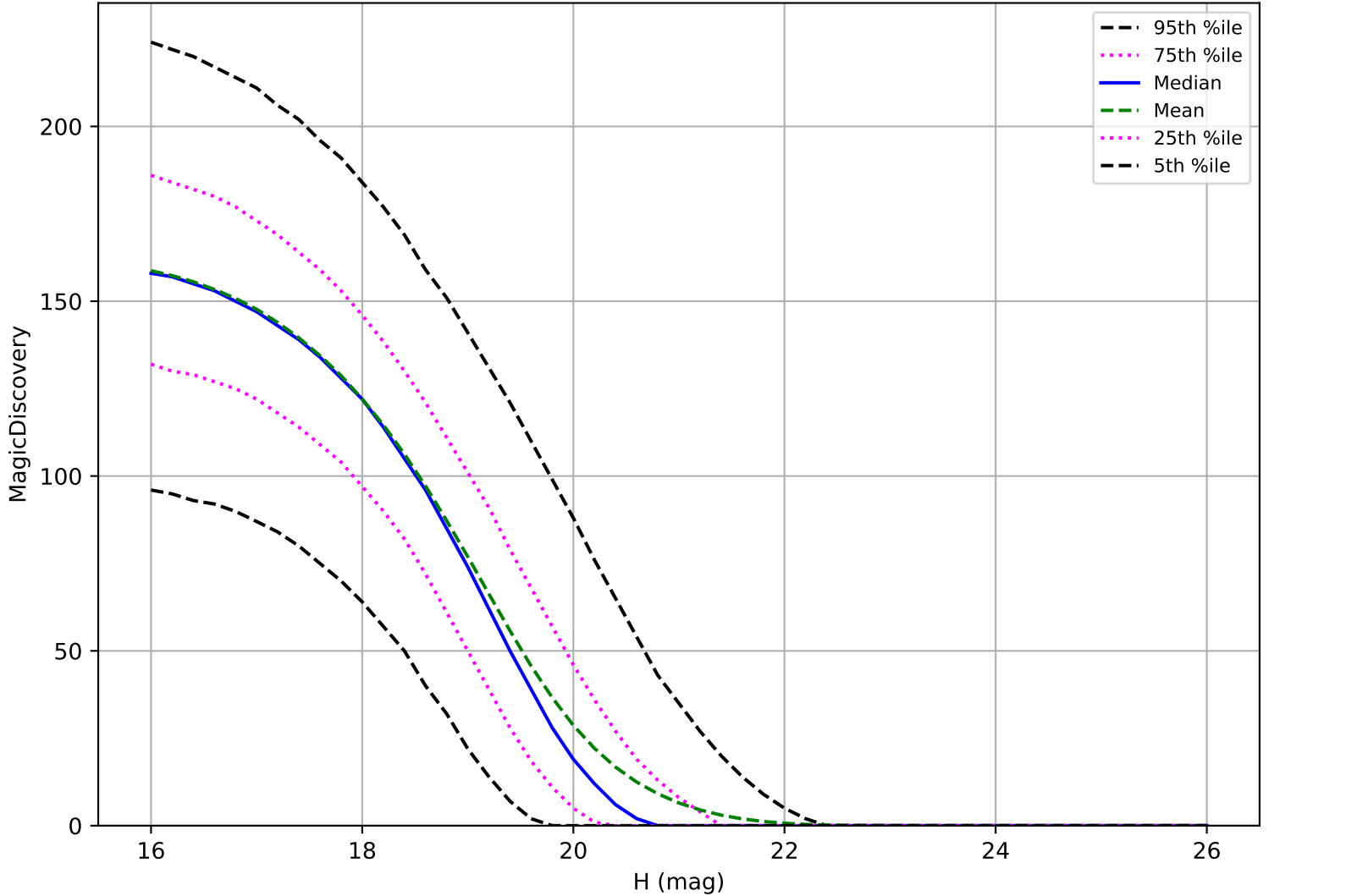
roll_uniform_early_half_accordion1_mjdp0_v3.4_10yrs: MBA 6 detections in 60 nights detection loss
