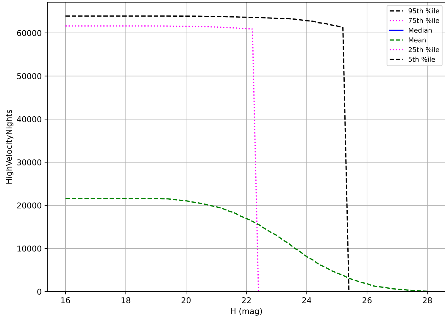
roll_uniform_early_half_accordion1_mjdp0_v3.4_10yrs: PHA High velocity pair detection loss
