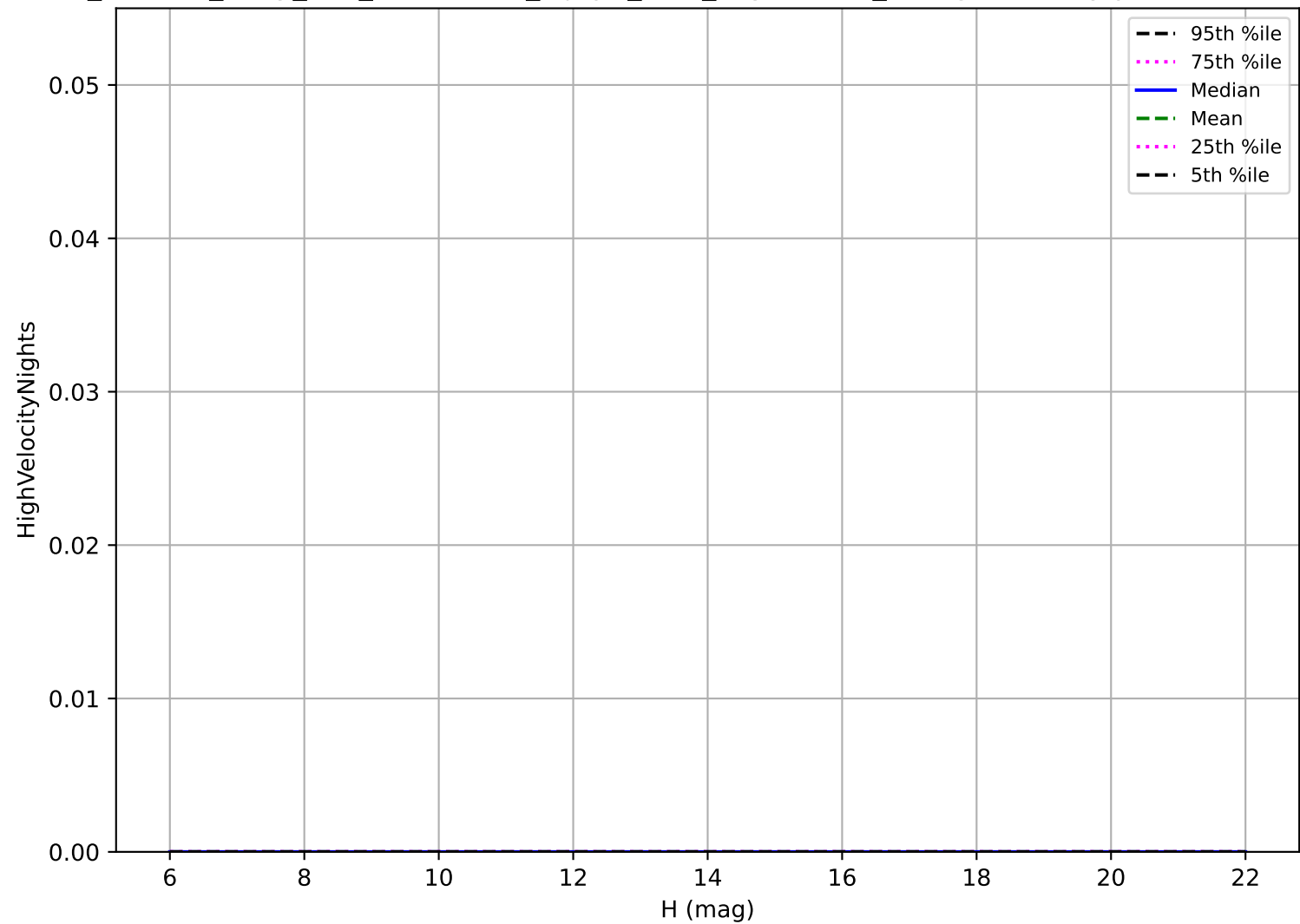
roll_uniform_early_half_accordion1_mjdp0_v3.4_10yrs: OCC_r5 High velocity pair detection loss
