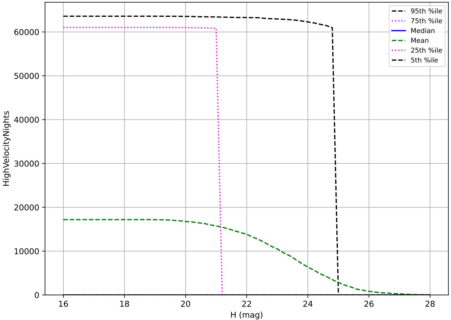
roll_uniform_early_half_accordion1_mjdp0_v3.4_10yrs: NEO High velocity pair detection loss
