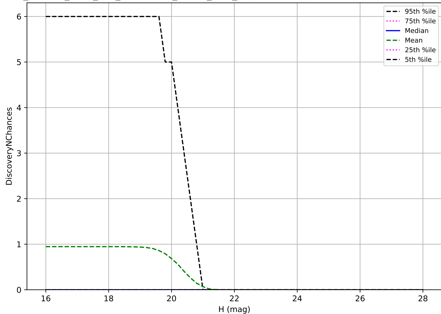
roll_uniform_early_half_accordion1_mjdp0_v3.4_10yrs: Vatira 3 pairs in 15 nights detection loss
