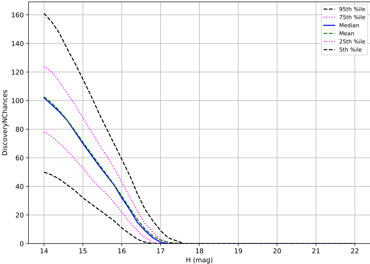
roll_uniform_early_half_accordion1_mjdp0_v3.4_10yrs: Trojan 3 pairs in 15 nights detection loss
