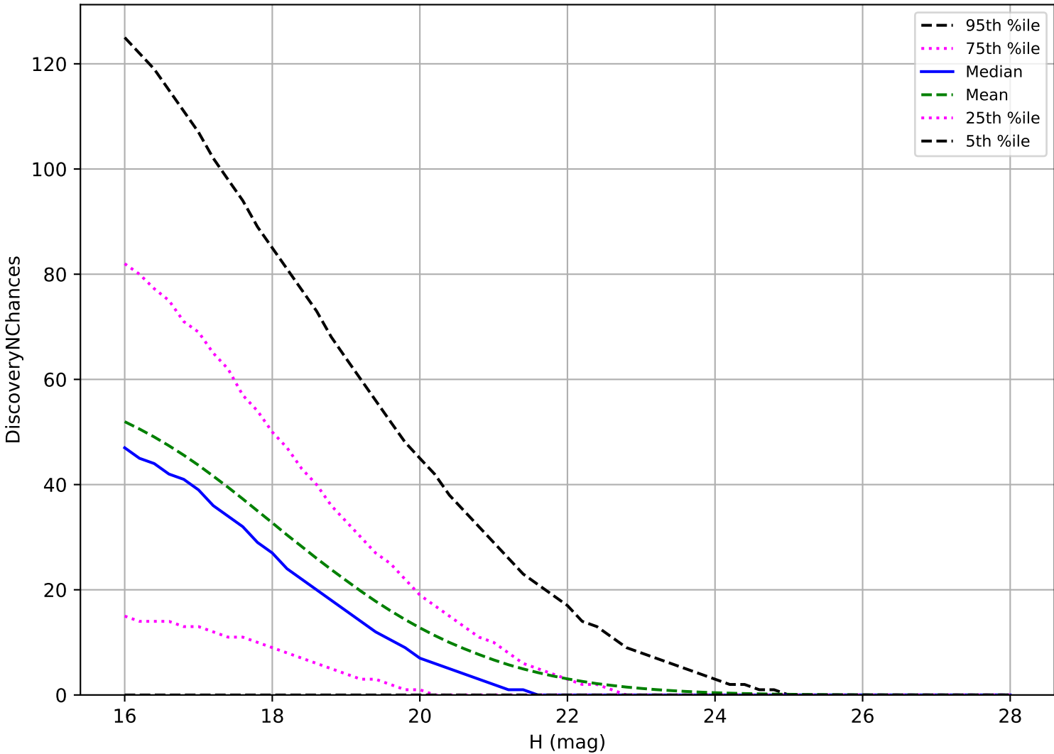
roll_uniform_early_half_accordion1_mjdp0_v3.4_10yrs: PHA 3 pairs in 15 nights detection loss
