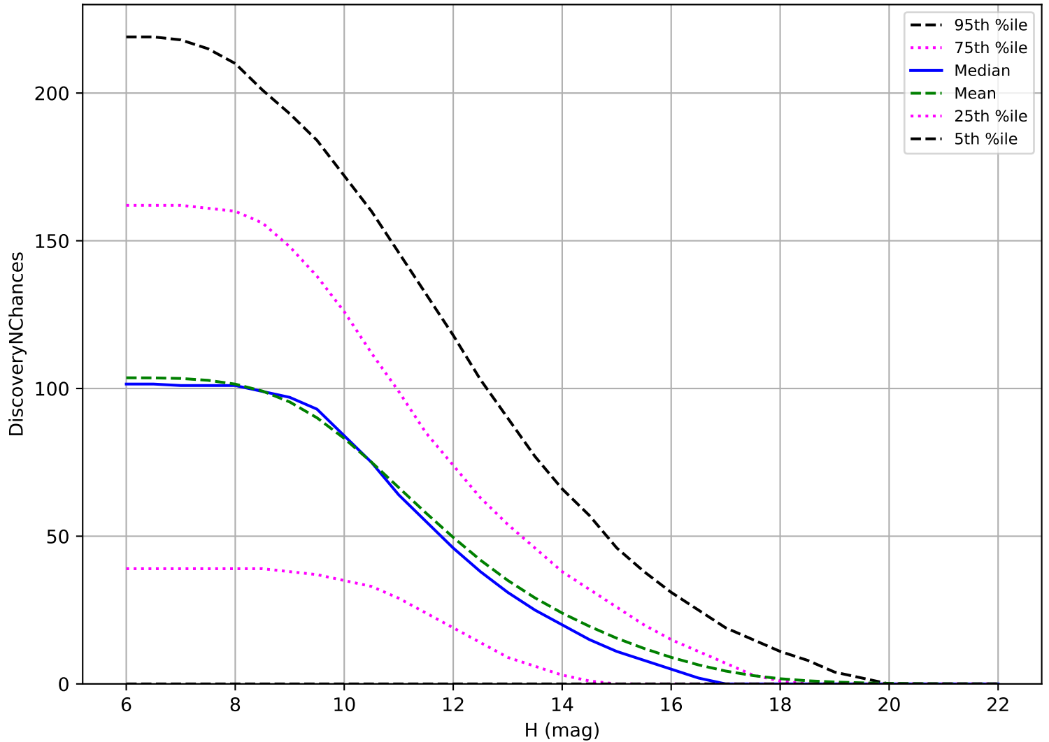
roll_uniform_early_half_accordion1_mjdp0_v3.4_10yrs: OCC_r5 3 pairs in 15 nights detection loss
