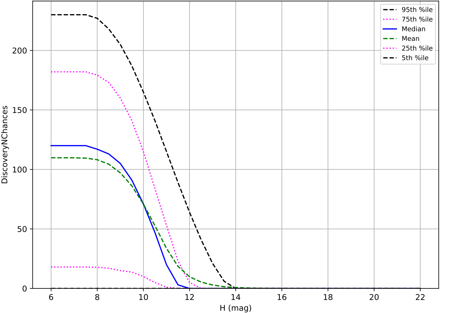
roll_uniform_early_half_accordion1_mjdp0_v3.4_10yrs: OCC_r20 3 pairs in 15 nights detection loss
