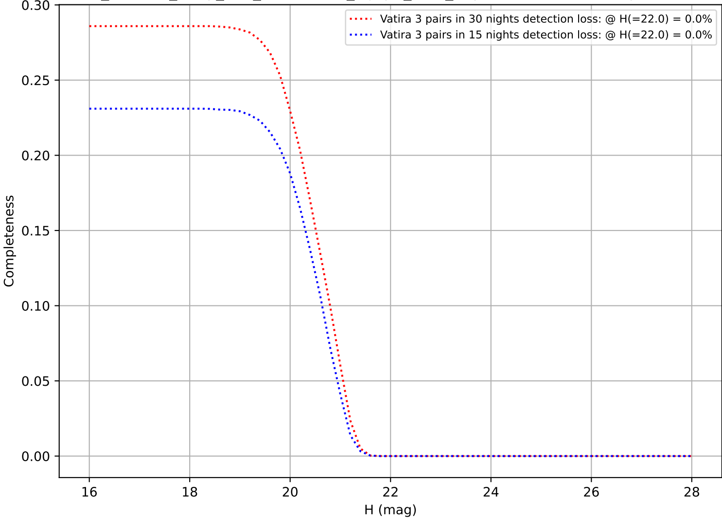
roll_uniform_early_half_accordion1_mjdp0_v3.4_10yrs: DifferentialCompleteness
