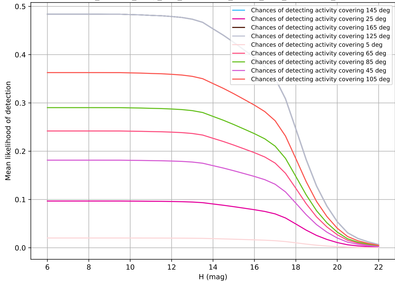
roll_uniform_early_half_accordion1_mjdp0_v3.4_10yrs OCC_r5
