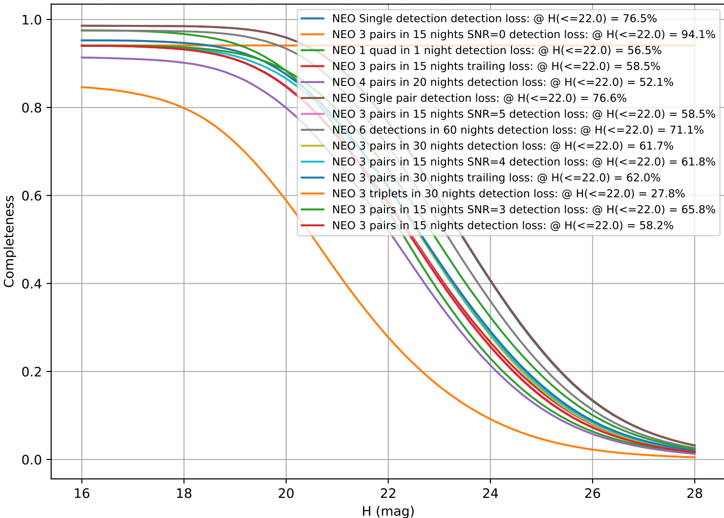
roll_uniform_early_half_accordion1_mjdp0_v3.4_10yrs: CumulativeCompleteness
