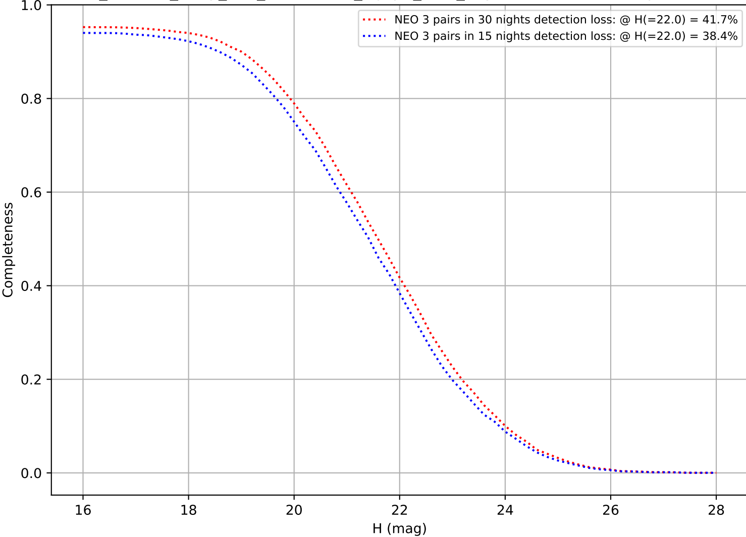
roll_uniform_early_half_accordion1_mjdp0_v3.4_10yrs: DifferentialCompleteness
