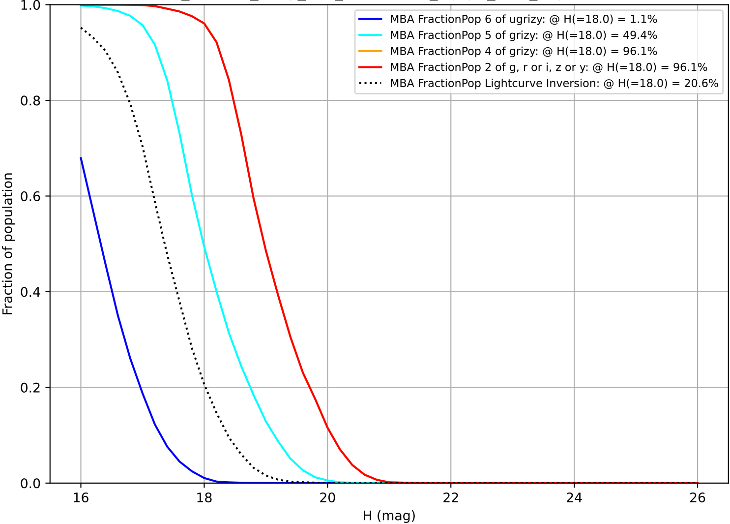
roll_uniform_early_half_accordion1_mjdp0_v3.4_10yrs MBA
