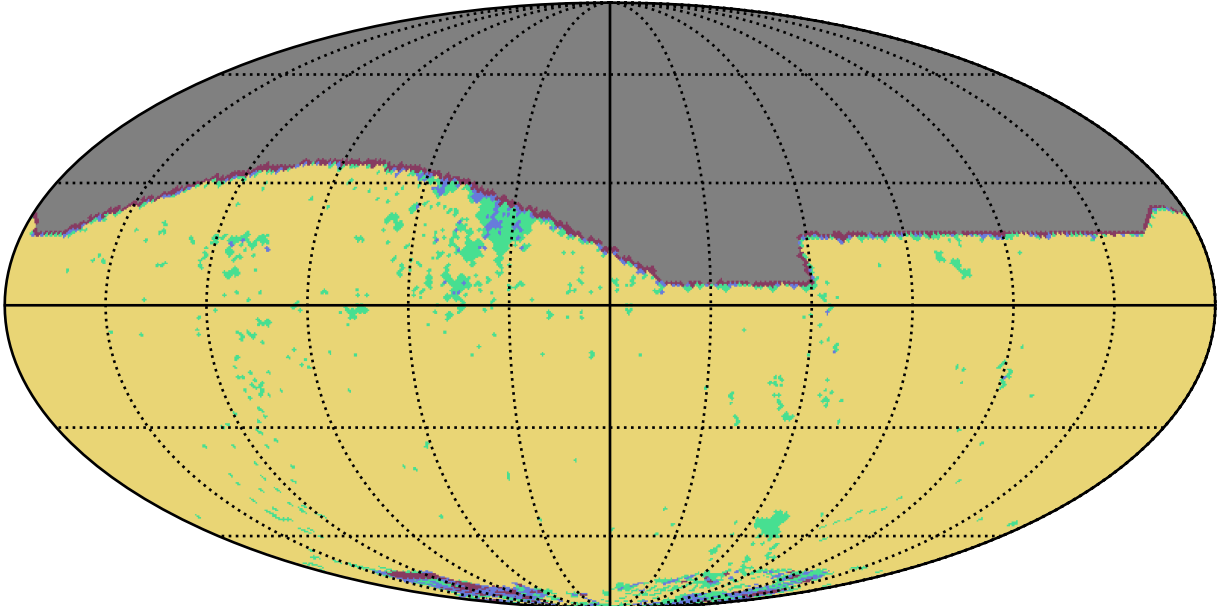
roll_uniform_early_half_accordion1_mjdp0_v3.4_10yrs i band: YearCoverage night
