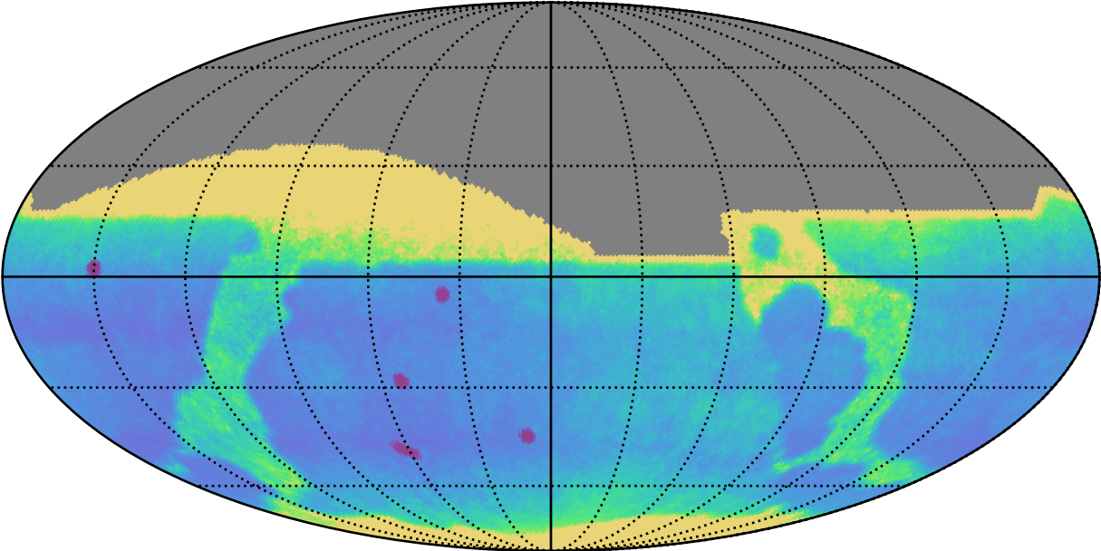
roll_uniform_early_half_accordion1_mjdp0_v3.4_10yrs : Proper Motion Uncert @ 24.0
