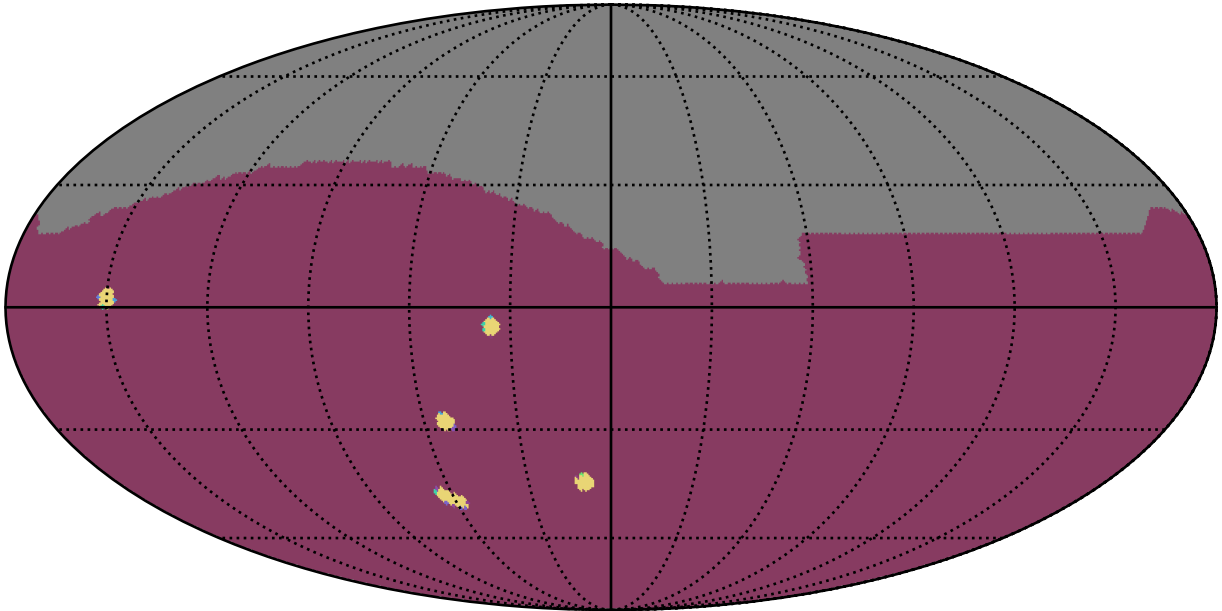
roll_uniform_early_half_accordion1_mjdp0_v3.4_10yrs : NumberOfQuickRevisits
