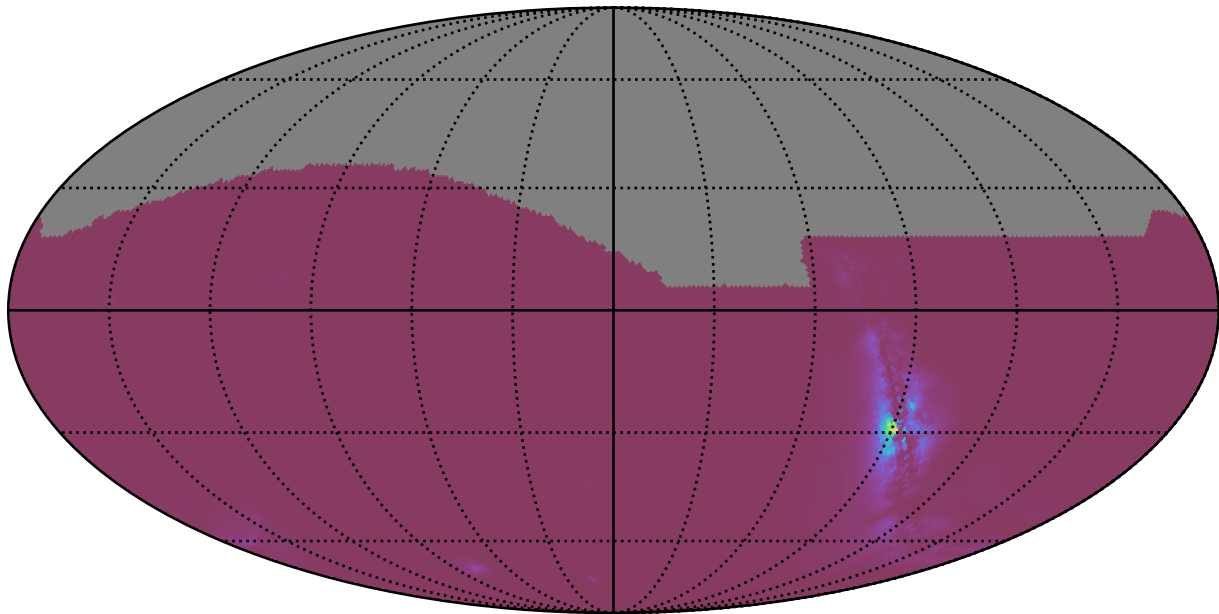
roll_uniform_early_half_accordion1_mjdp0_v3.4_10yrs : NlcPoints
