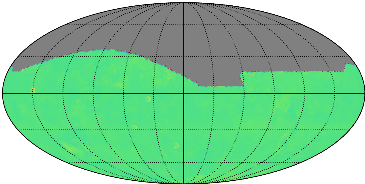
roll_uniform_early_half_accordion1_mjdp0_v3.4_10yrs i: Kuiper rotTelPos
