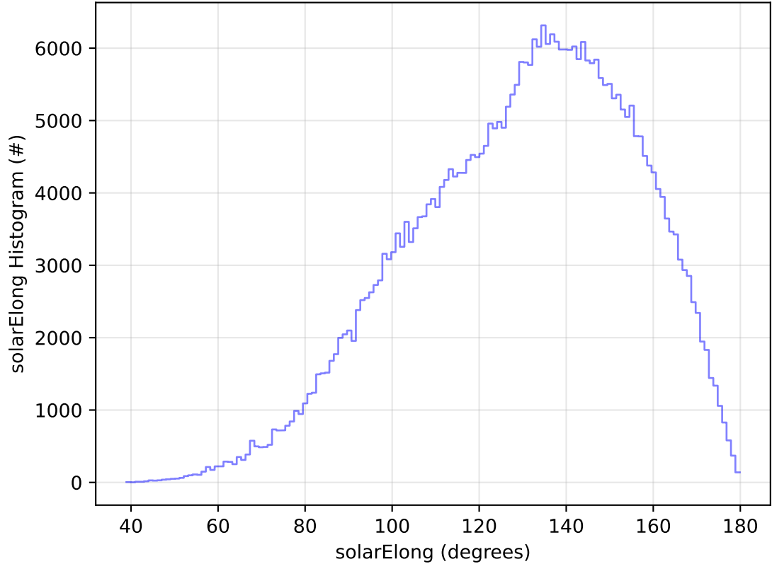
roll_uniform_early_half_accordion1_mjdp0_v3.4_10yrs WFD y band: solarElong Histogram
