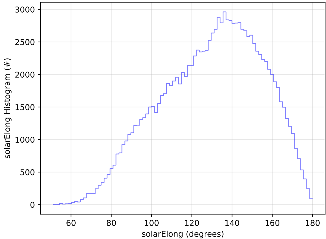
roll_uniform_early_half_accordion1_mjdp0_v3.4_10yrs WFD u band: solarElong Histogram
