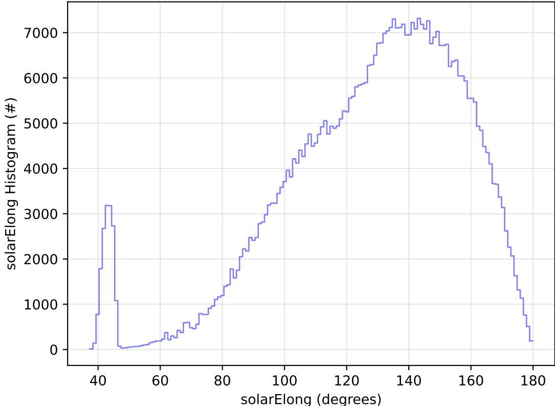
roll_uniform_early_half_accordion1_mjdp0_v3.4_10yrs WFD r band: solarElong Histogram
