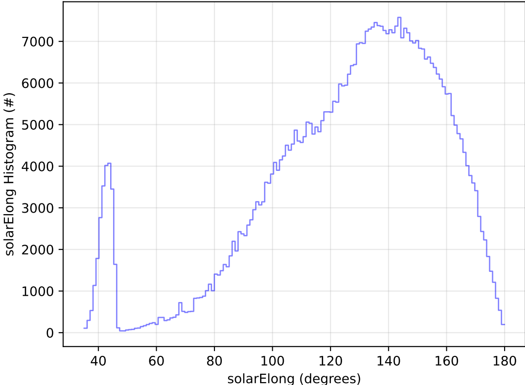
roll_uniform_early_half_accordion1_mjdp0_v3.4_10yrs WFD i band: solarElong Histogram
