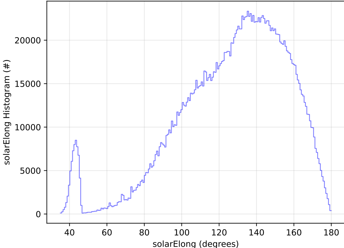
roll_uniform_early_half_accordion1_mjdp0_v3.4_10yrs WFD all bands: solarElong Histogram
