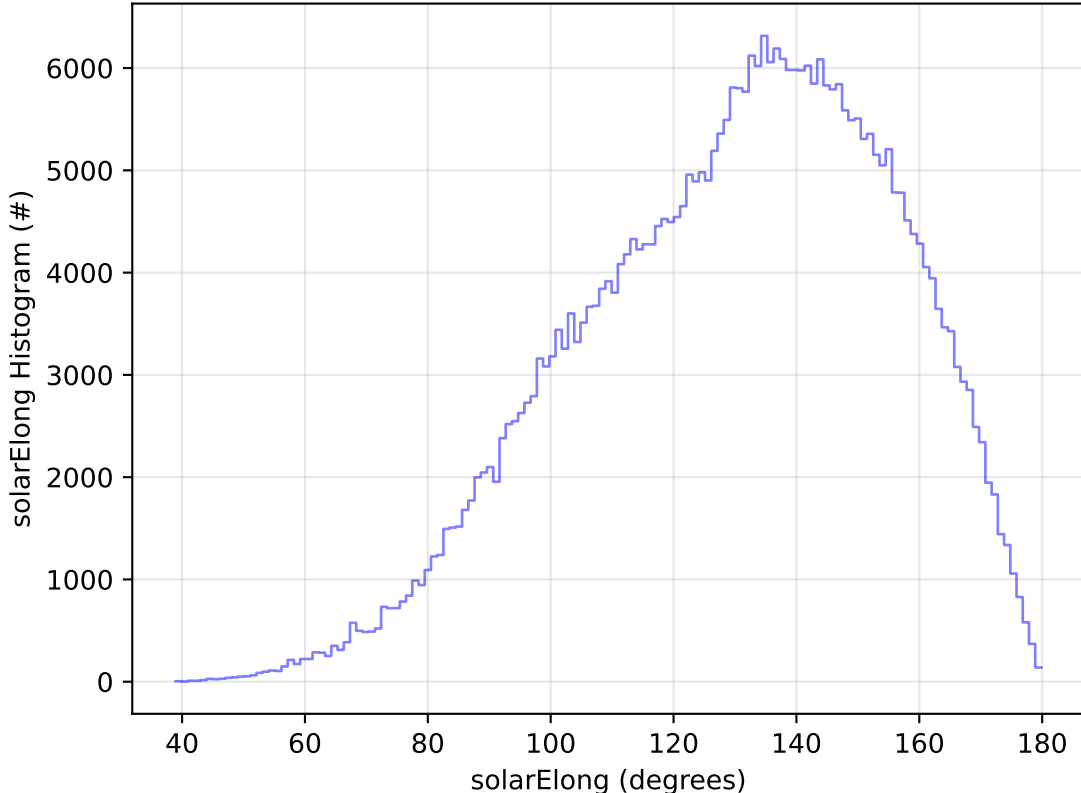
roll_uniform_early_half_accordion1_mjdp0_v3.4_10yrs All sky y band: solarElong Histogram
