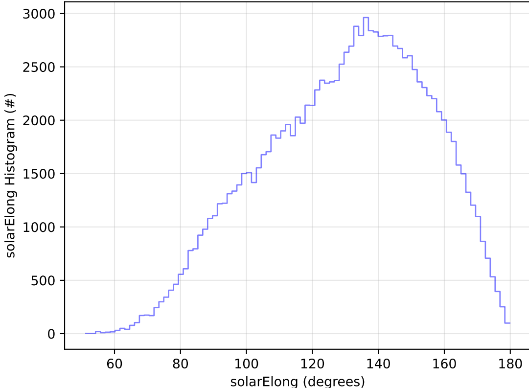
roll_uniform_early_half_accordion1_mjdp0_v3.4_10yrs All sky u band: solarElong Histogram
