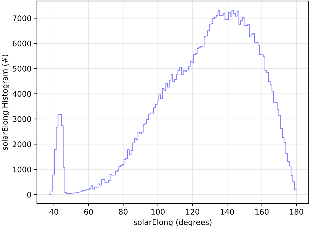
roll_uniform_early_half_accordion1_mjdp0_v3.4_10yrs All sky r band: solarElong Histogram
