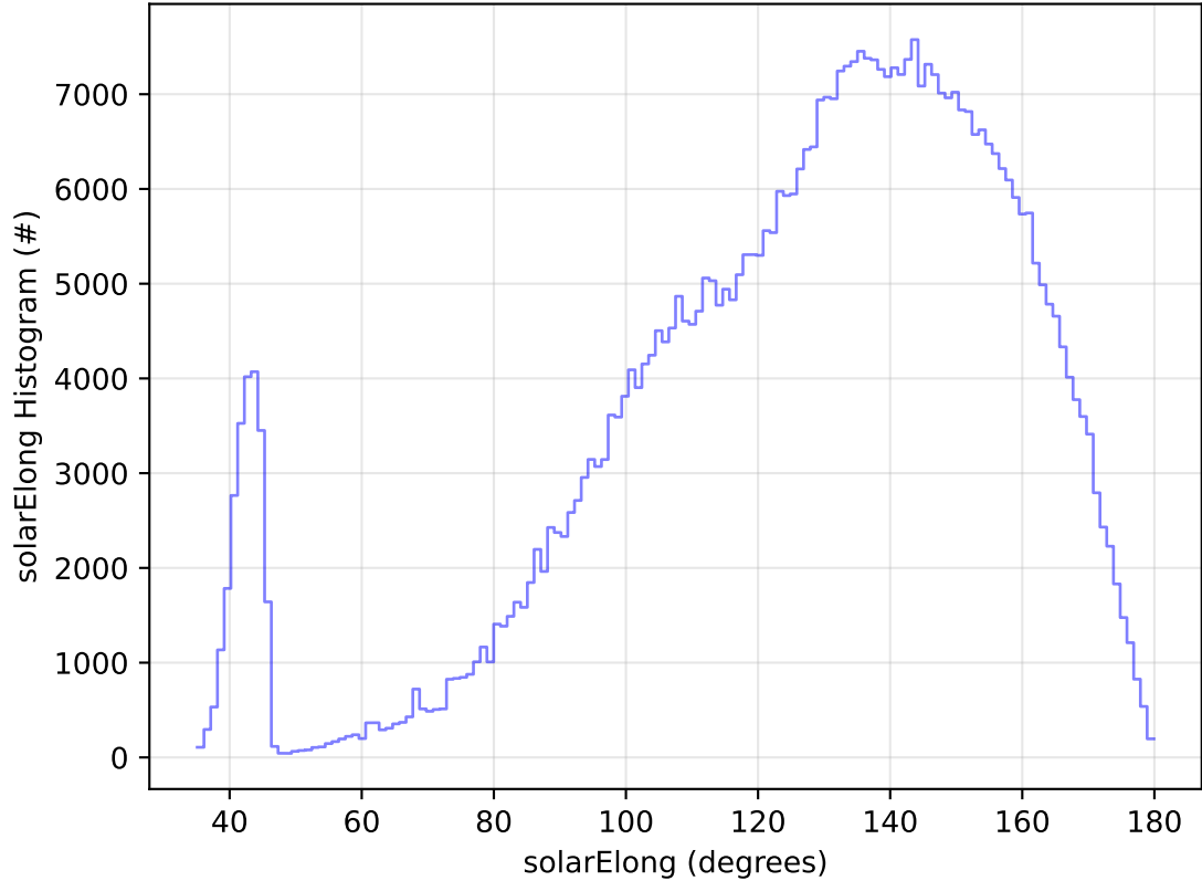
roll_uniform_early_half_accordion1_mjdp0_v3.4_10yrs All sky i band: solarElong Histogram
