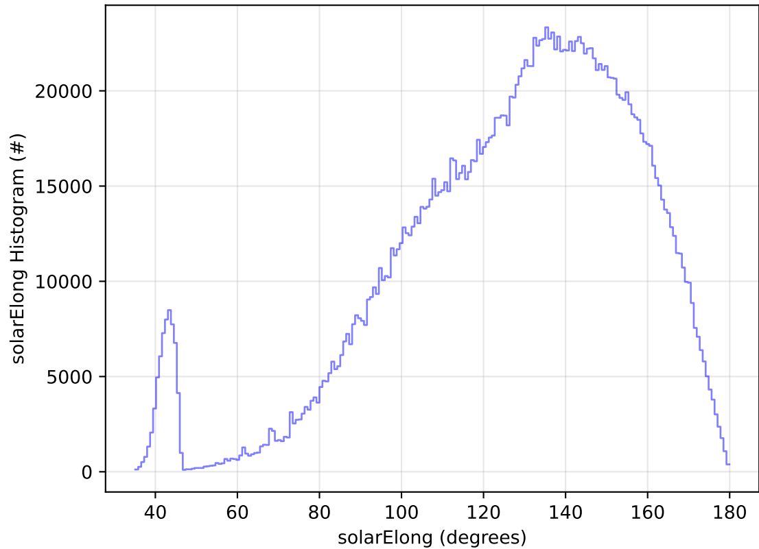
roll_uniform_early_half_accordion1_mjdp0_v3.4_10yrs All sky all bands: solarElong Histogram
