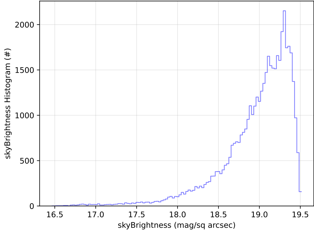
roll_uniform_early_half_accordion1_mjdp0_v3.4_10yrs Yr 1 z band: skyBrightness Histogram
